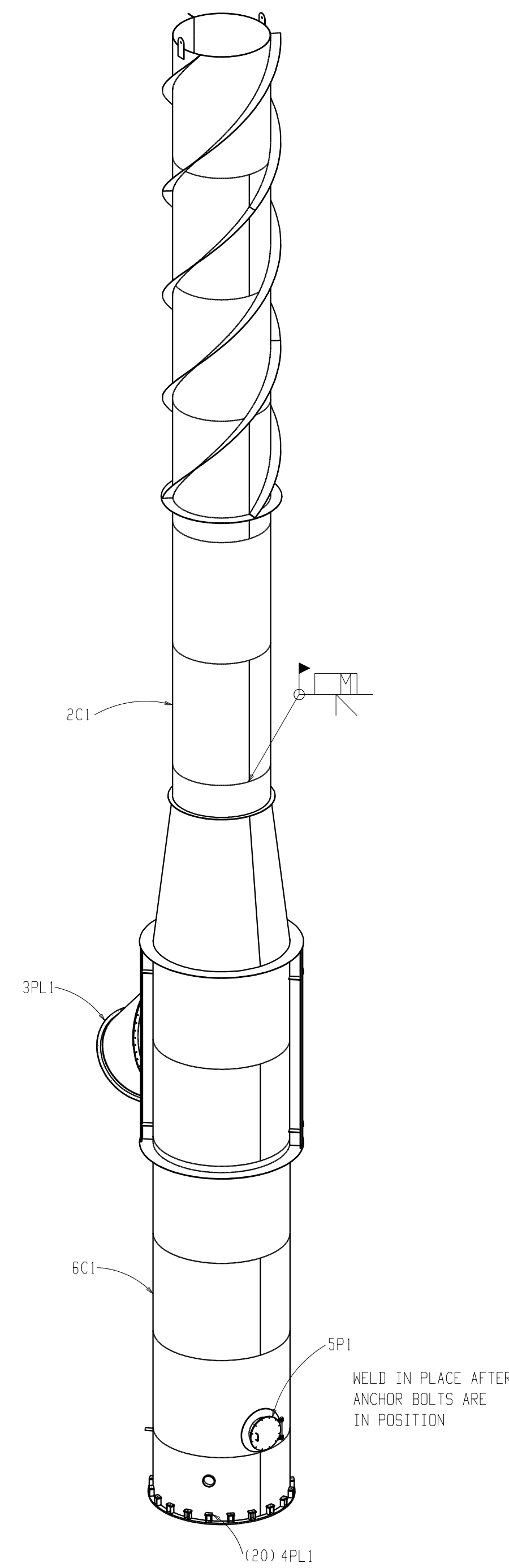
MDB FILTER STACK ISOMETRIC VIEW 2
