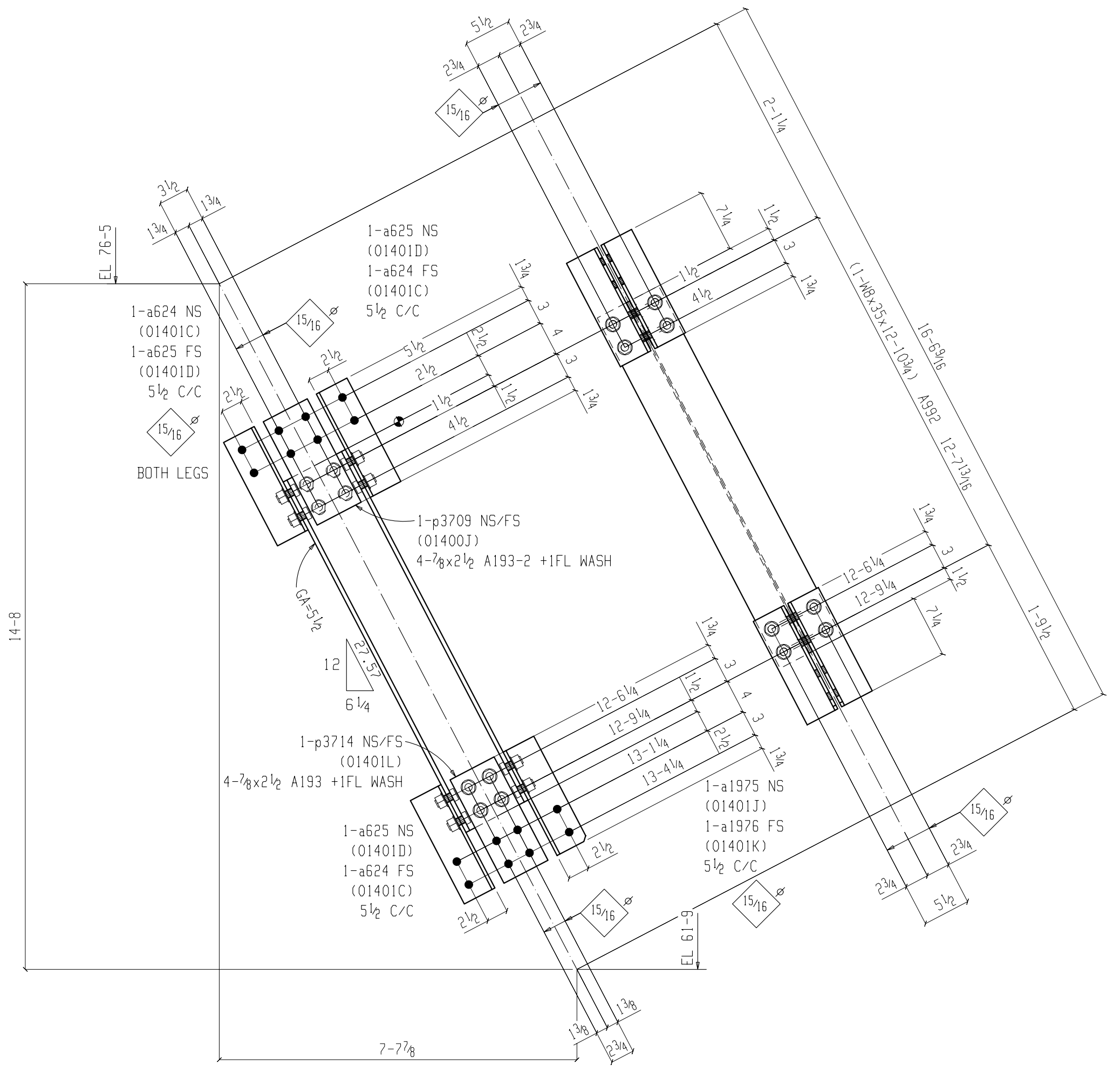
ONE VERTICAL BRACE 01401B
